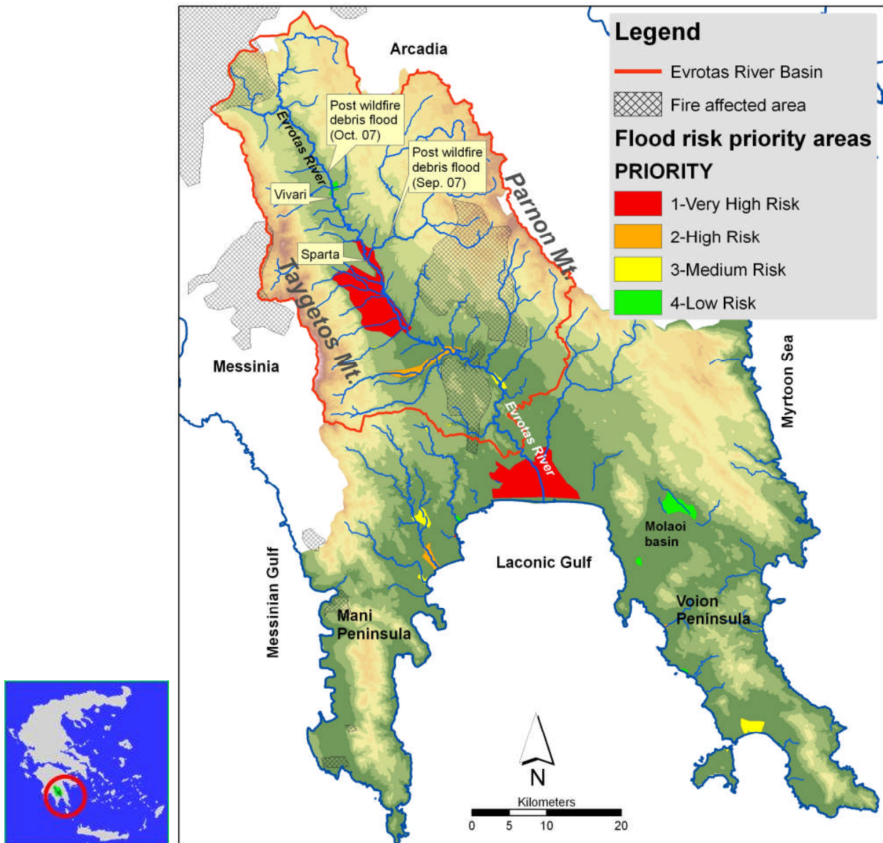
Fig1. Flood Risk Map of the study area [37]. The fire affected area of the 2007 wildfires is marked, as well as debris flood occurrences downstream, soonafter.
