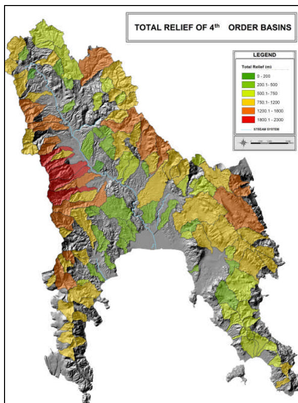
Fig2. Total Relief Map of 4 th order Basins
